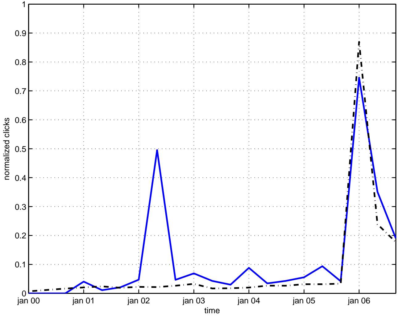
decay black hole
