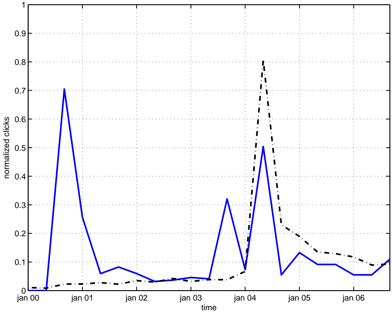
debye screening
