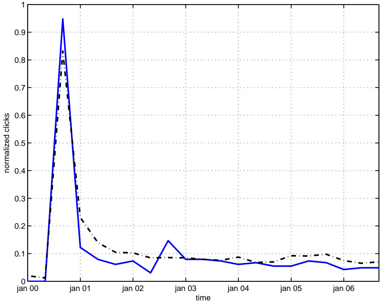
de sitter gauge field theory
