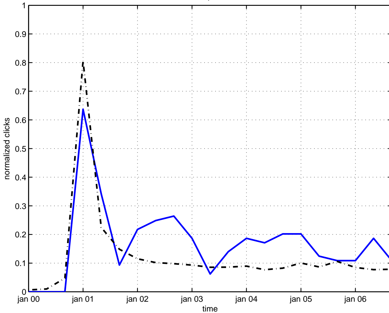
darwin potential
