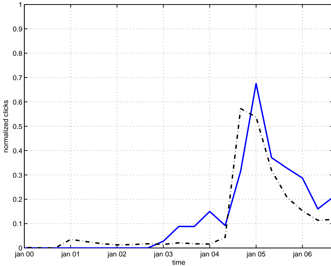
dark matter
