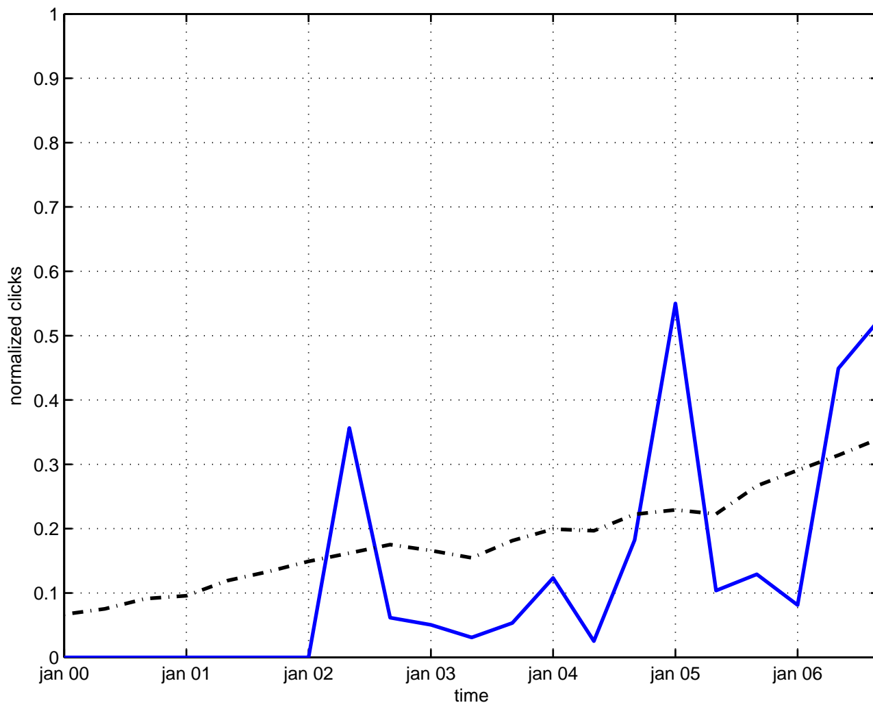
darboux transformation
