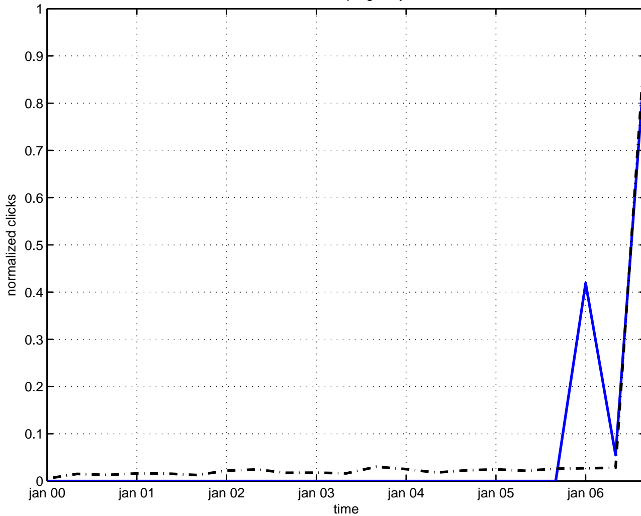
d-term supergravity
