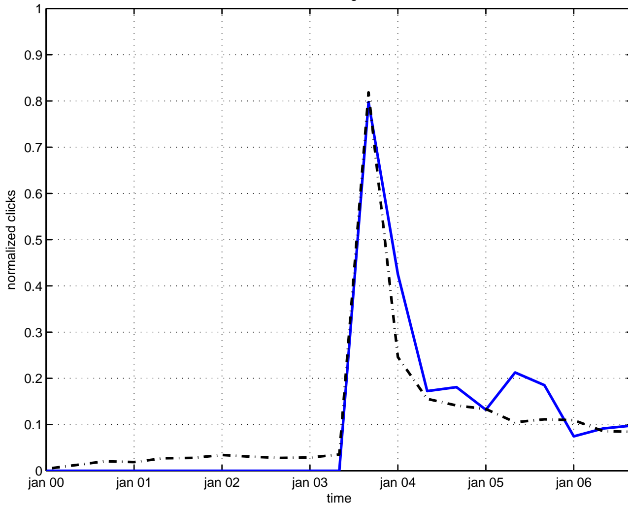
d-term string model
