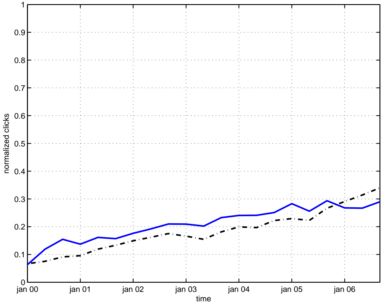
d-brane membrane model
