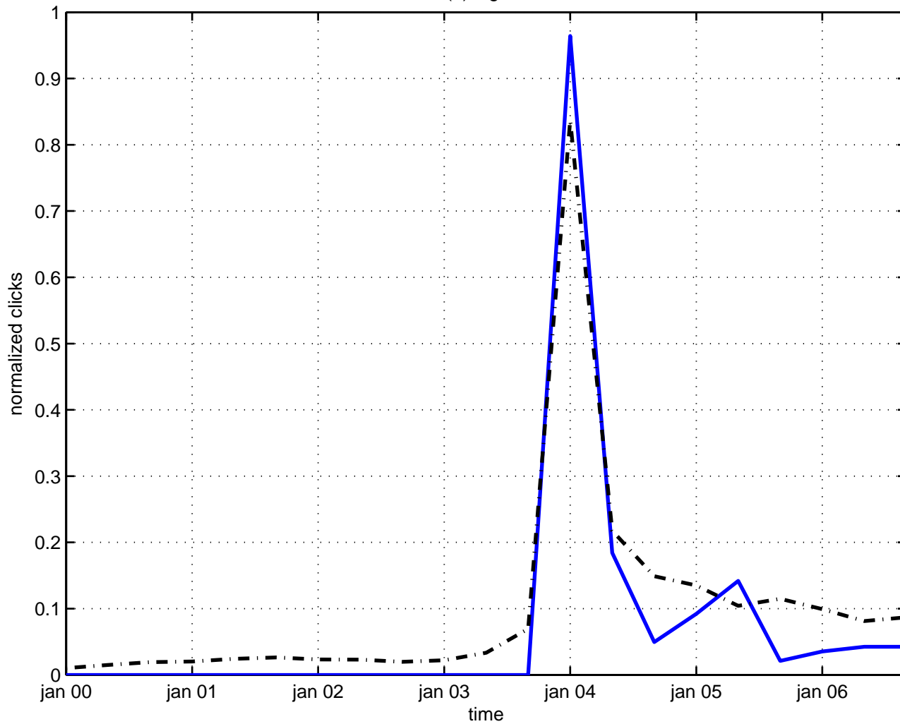
d(8) algebra
