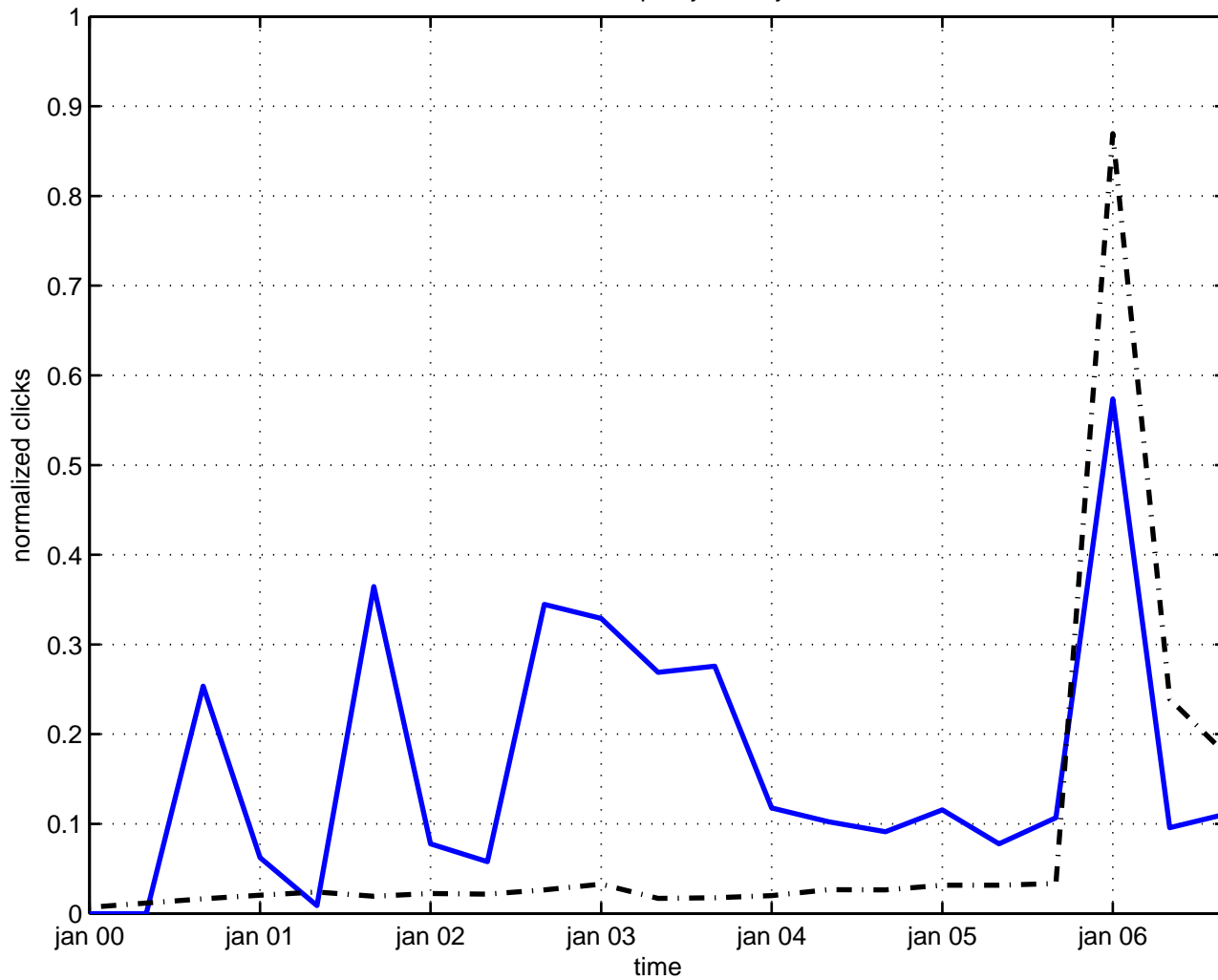
current supersymmetry
