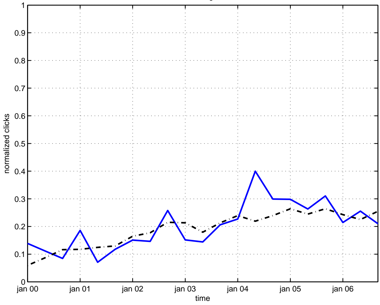
current algebra
