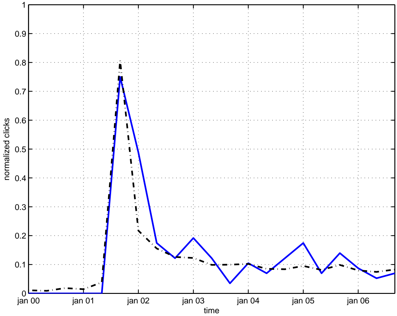
curci-ferrari model
