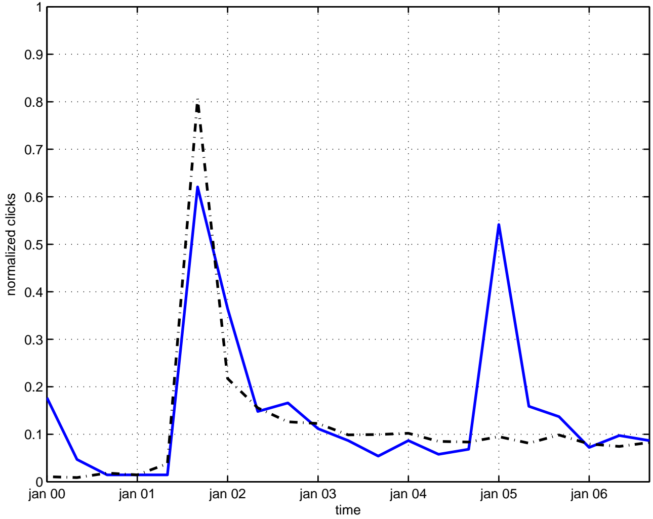
cumulant expansion
