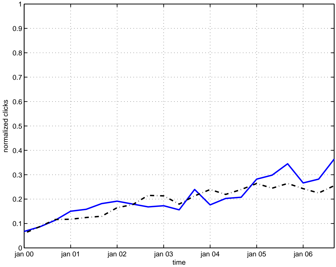
critical phenomena
