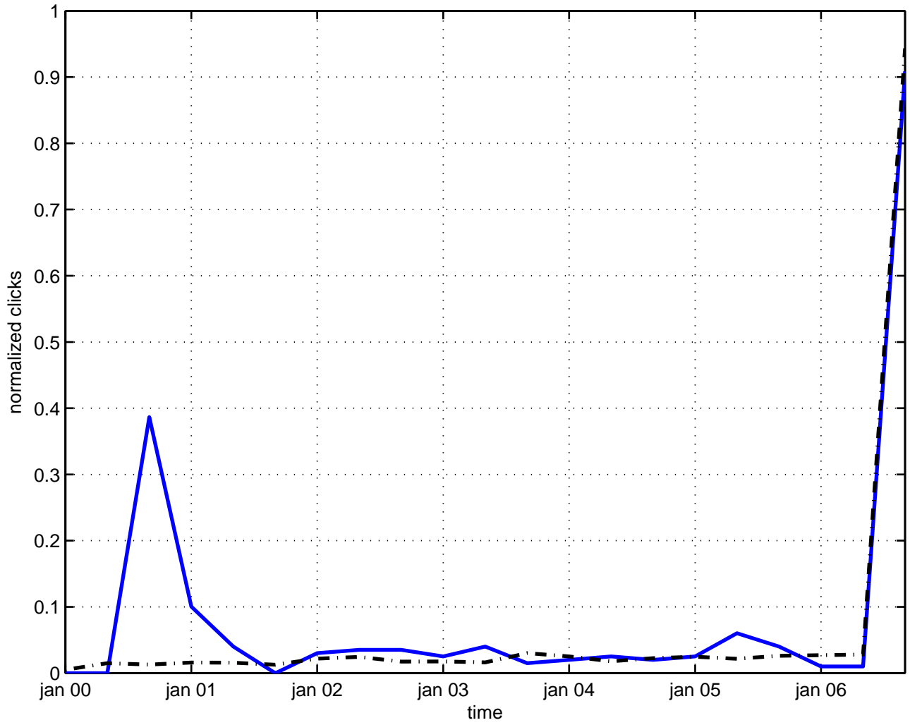
cpt symmetry breaking
