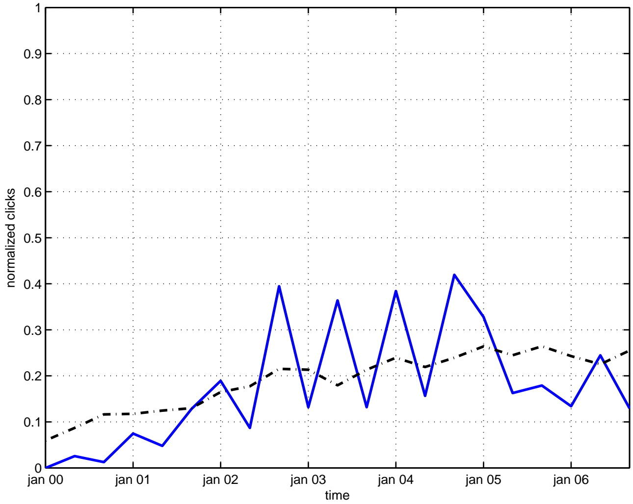
cpt invariance
