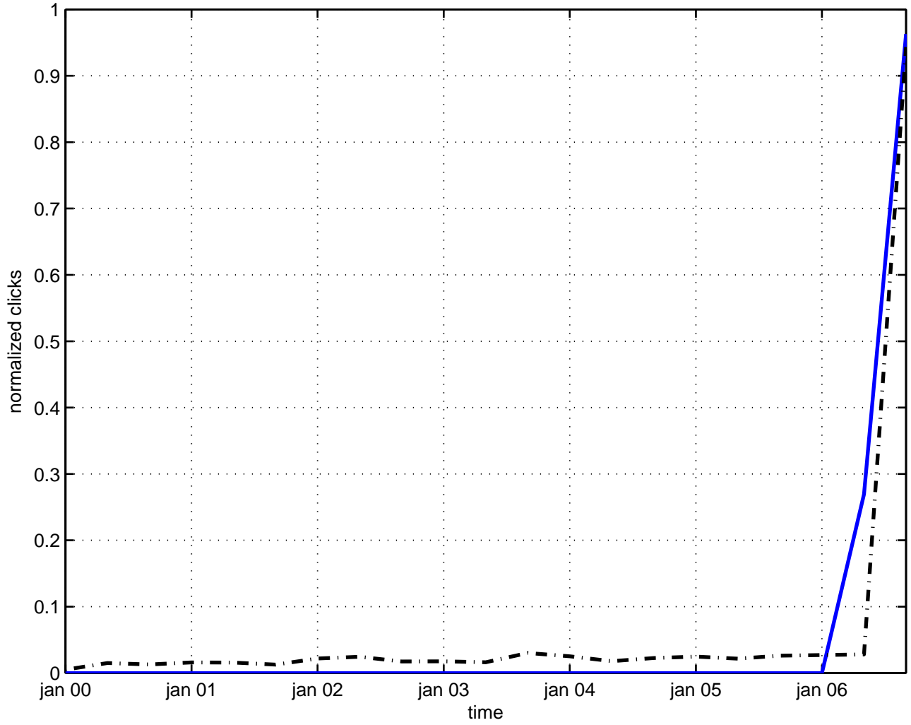
cp(n) model
