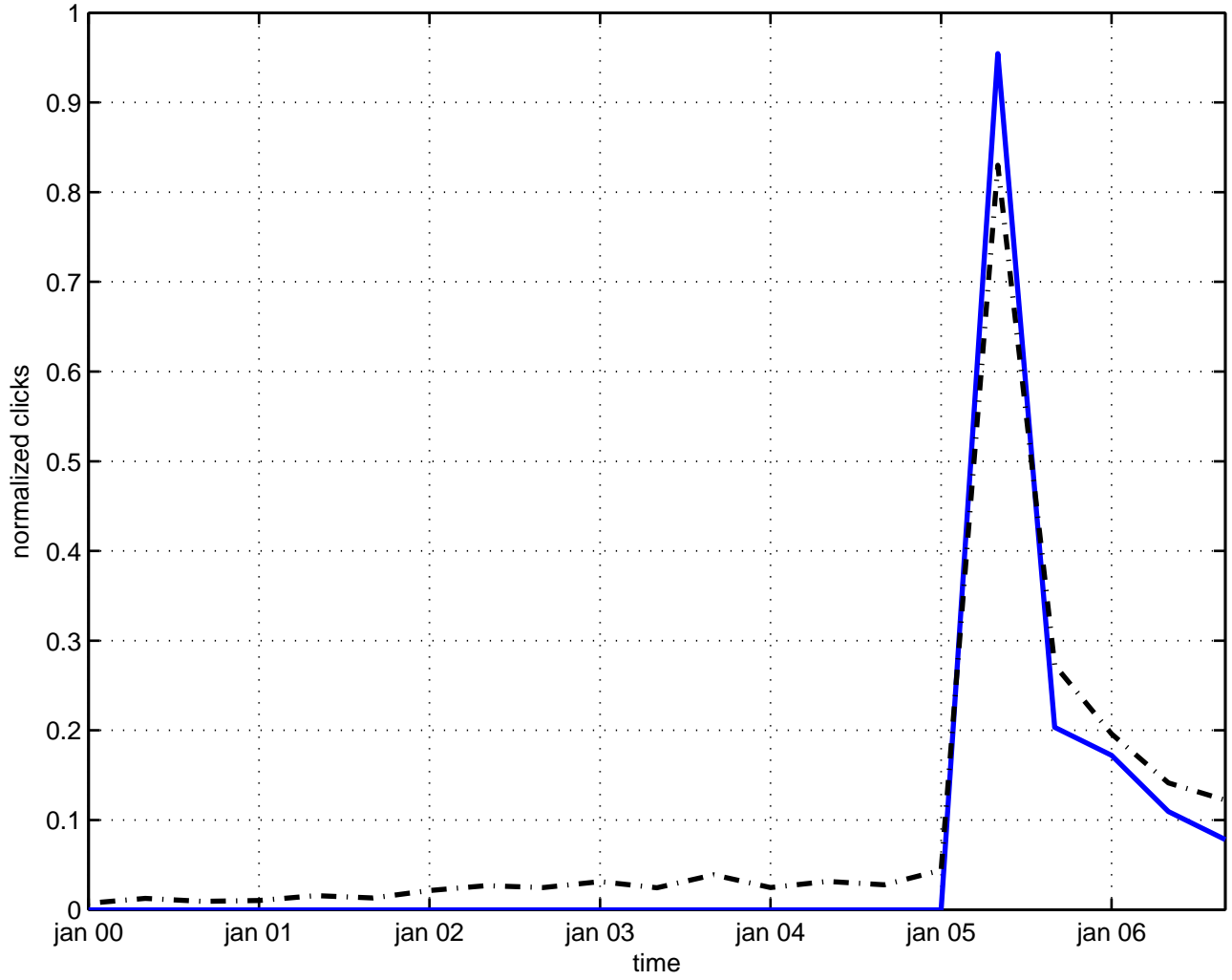
cp(1) model
