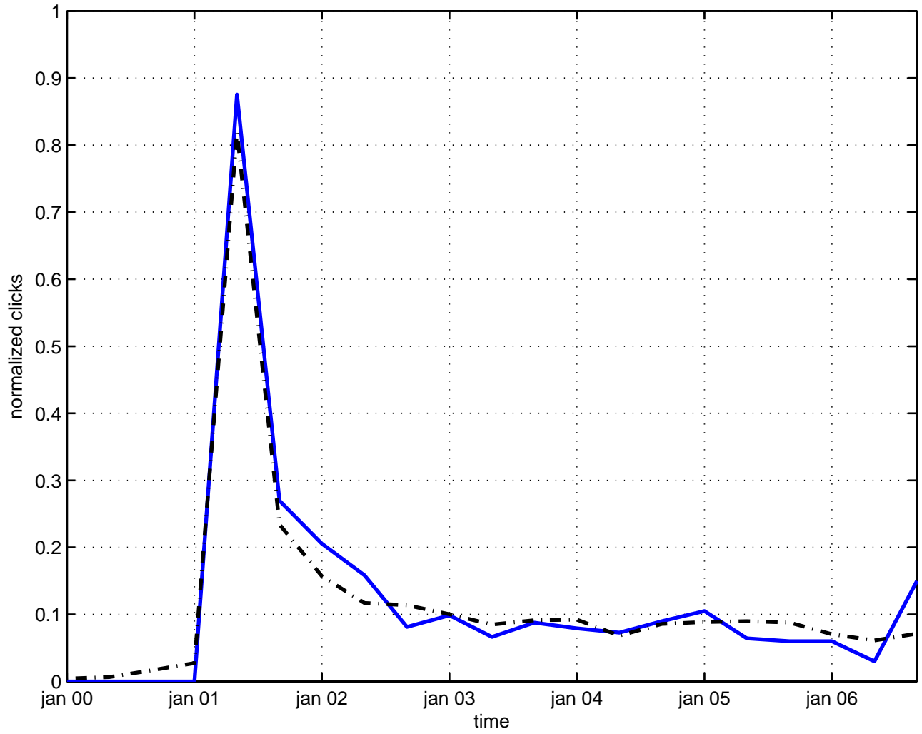
coupling string model
