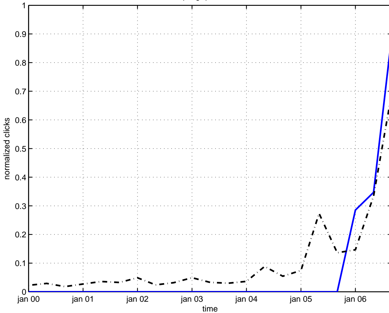
coupling quintessence
