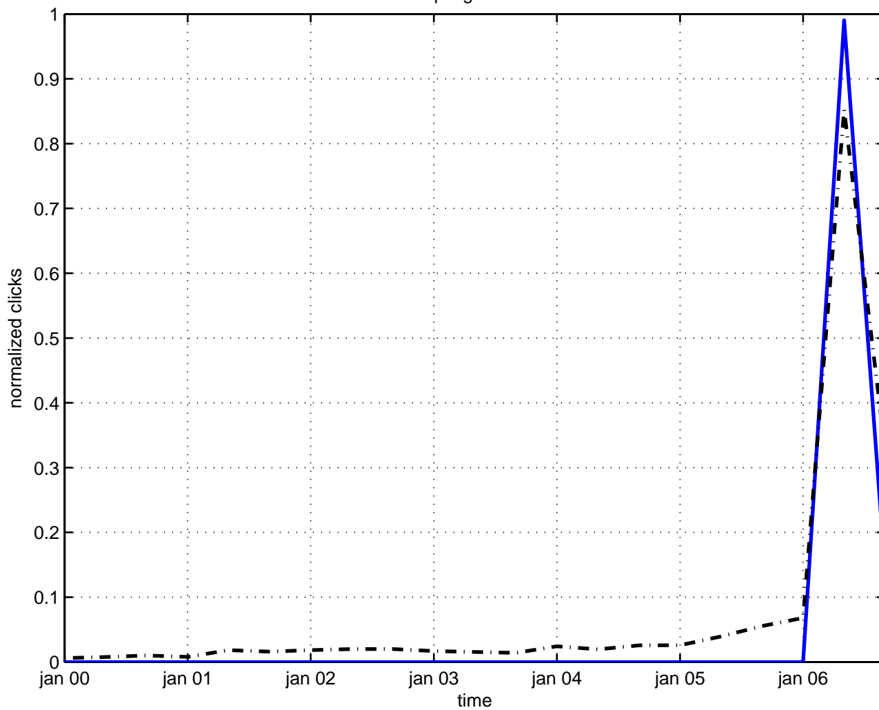
coupling neutrino
