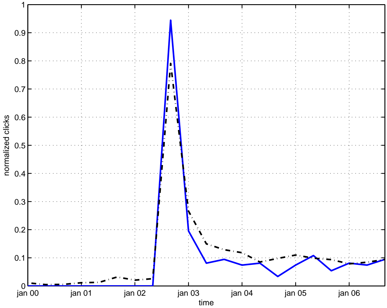
coupling multiplet
