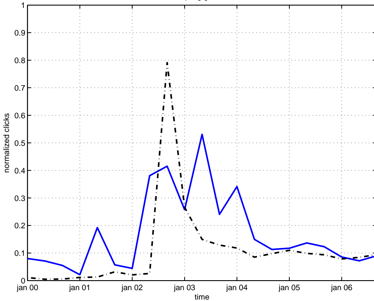
coupling graviton
