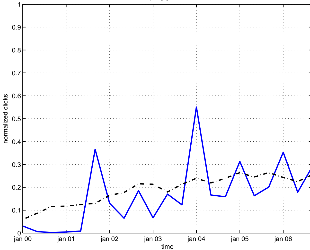
coupling gravitation
