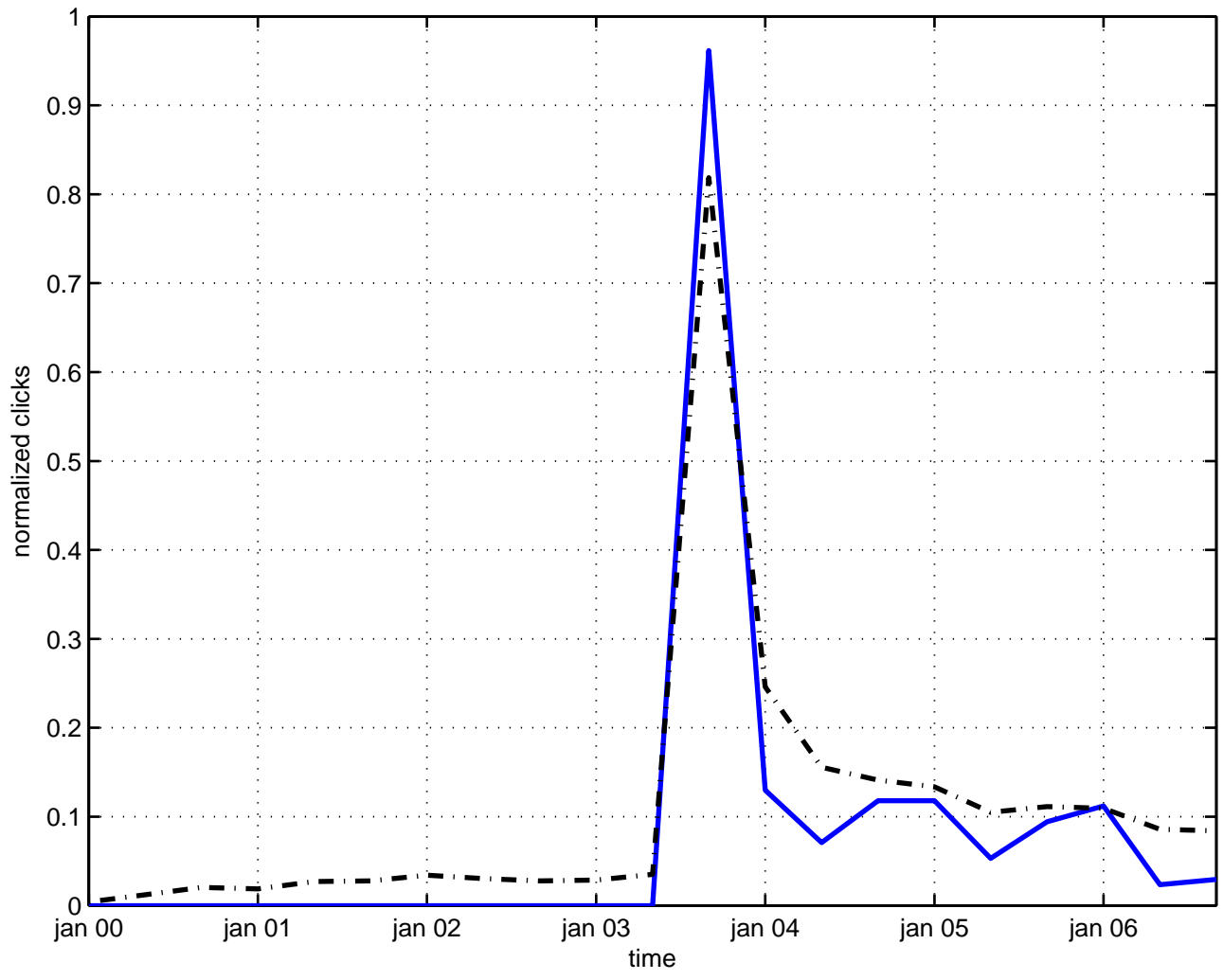
coulomb model
