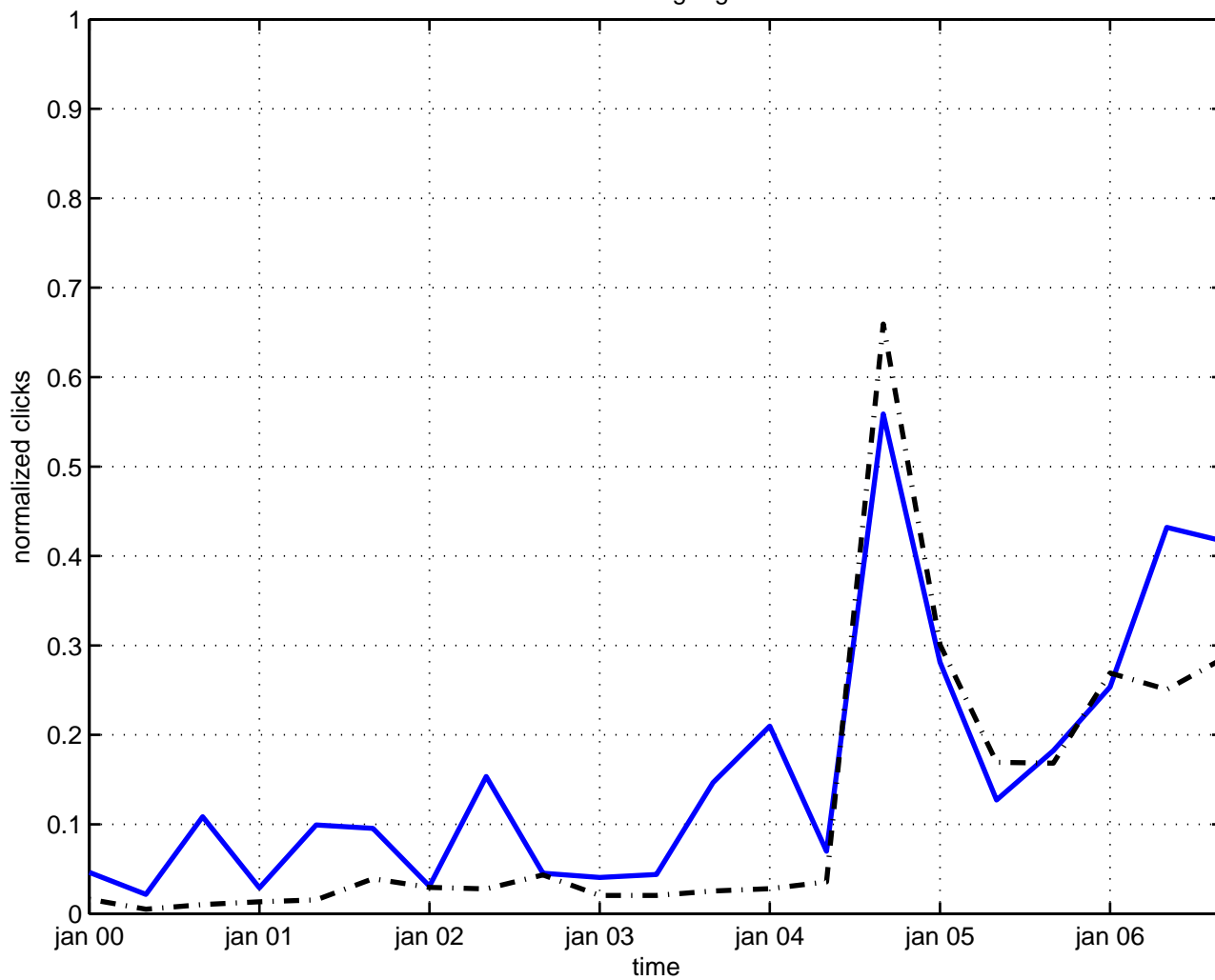
coulomb gauge
