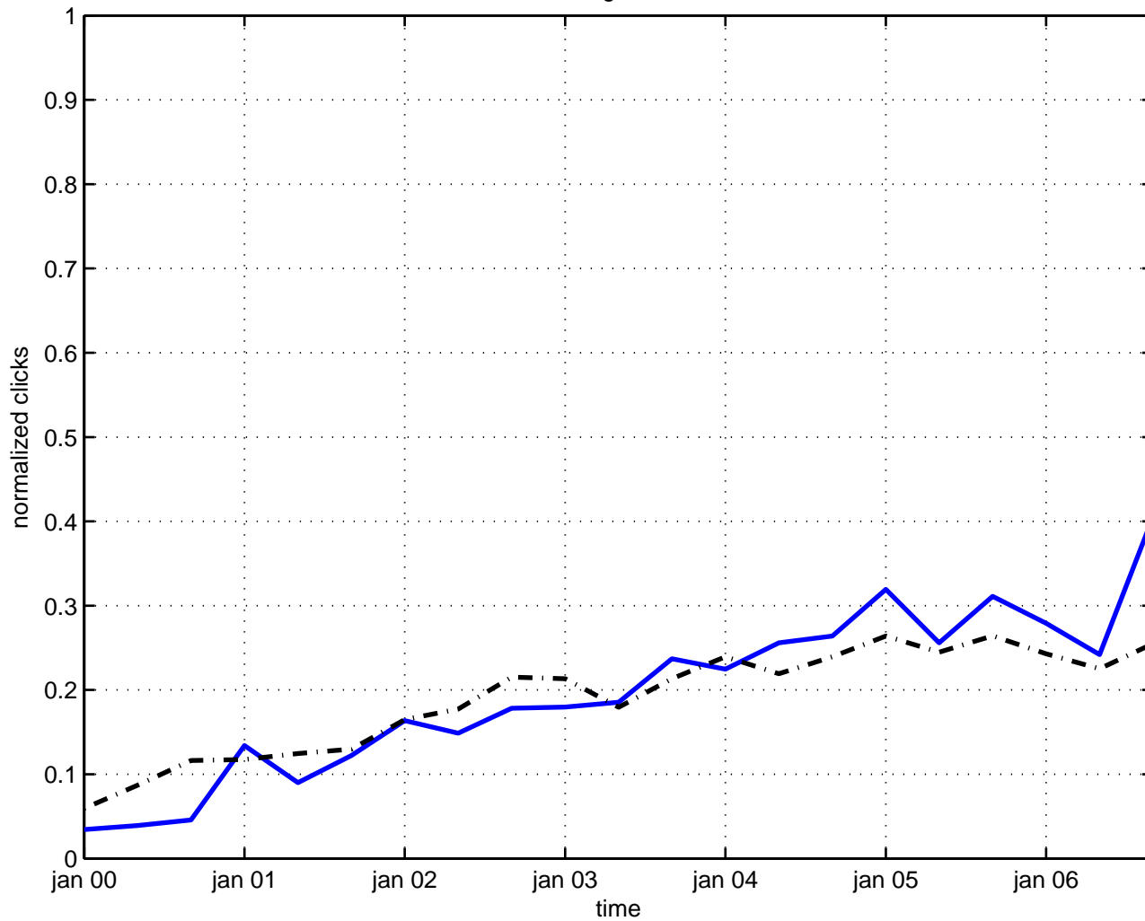
cosmological model
