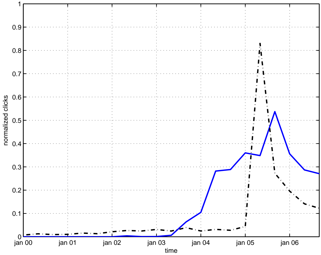
cosmic string
