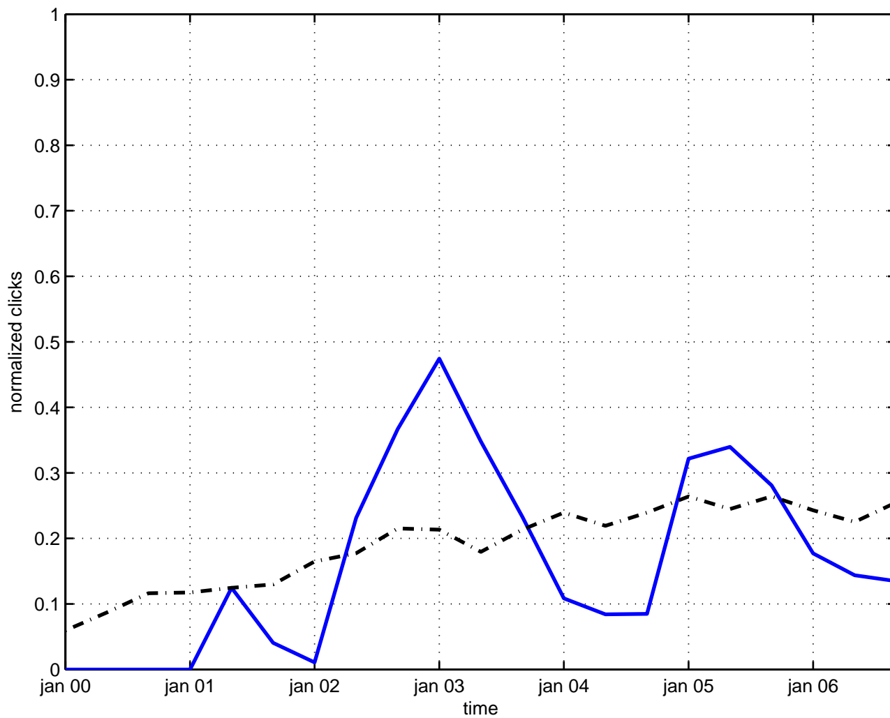
cosmic radiation
