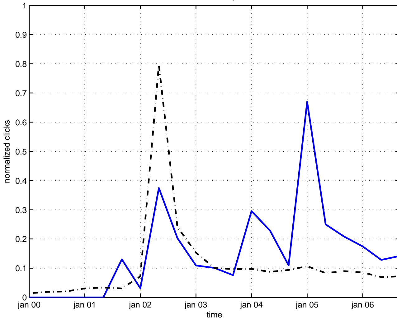
cosmic radiation photon
