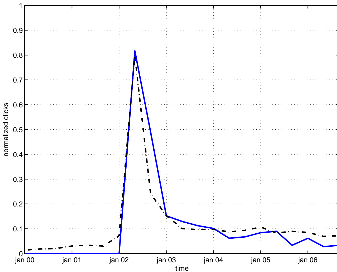
cosmic radiation neutrino
