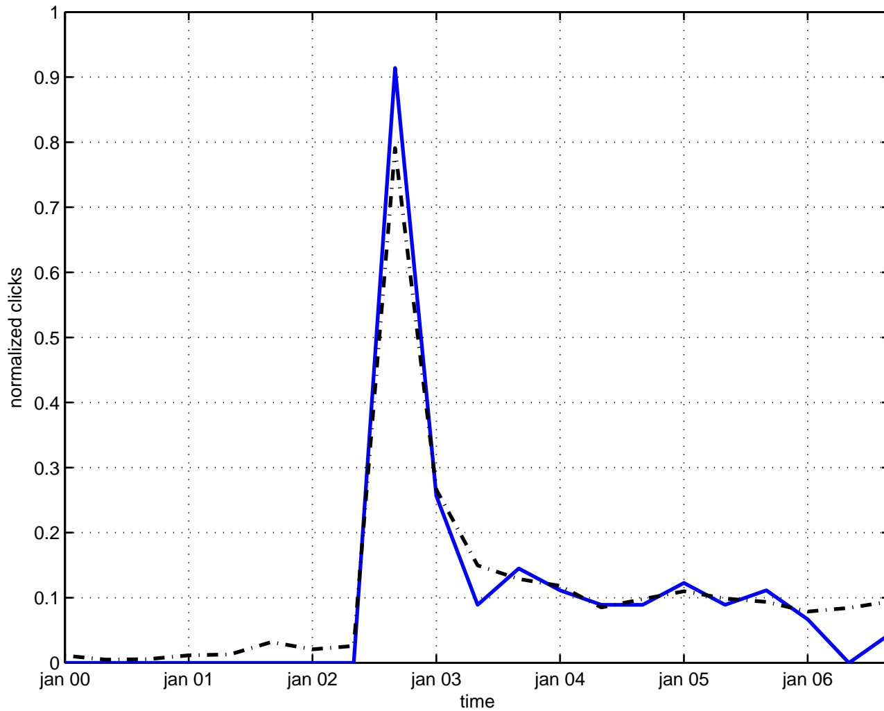
cosmic radiation hadron
