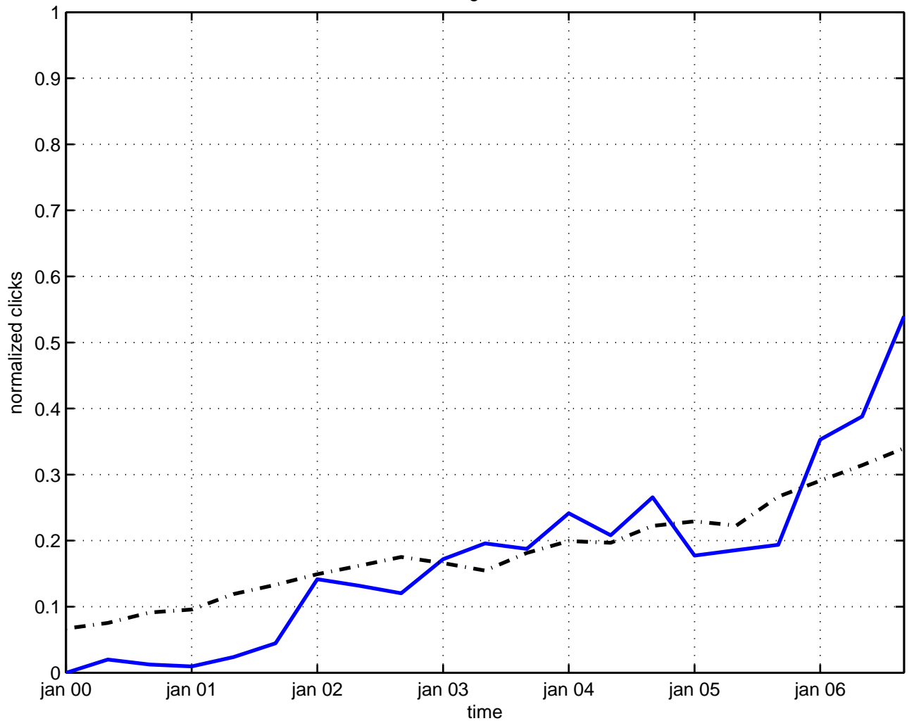
cosmic background radiation
