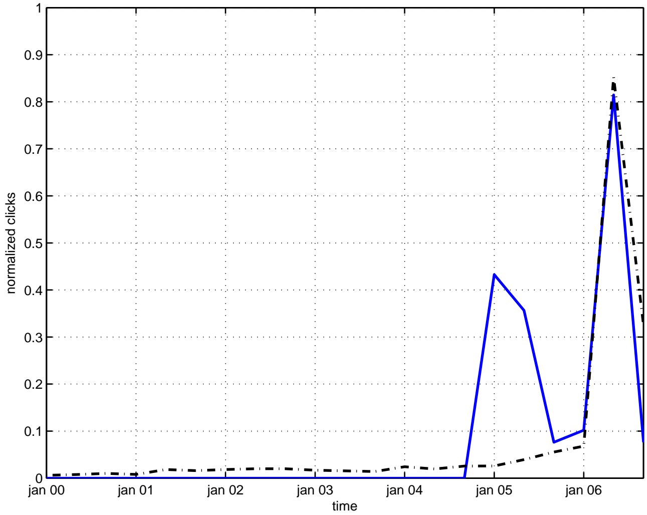
correlation polarization
