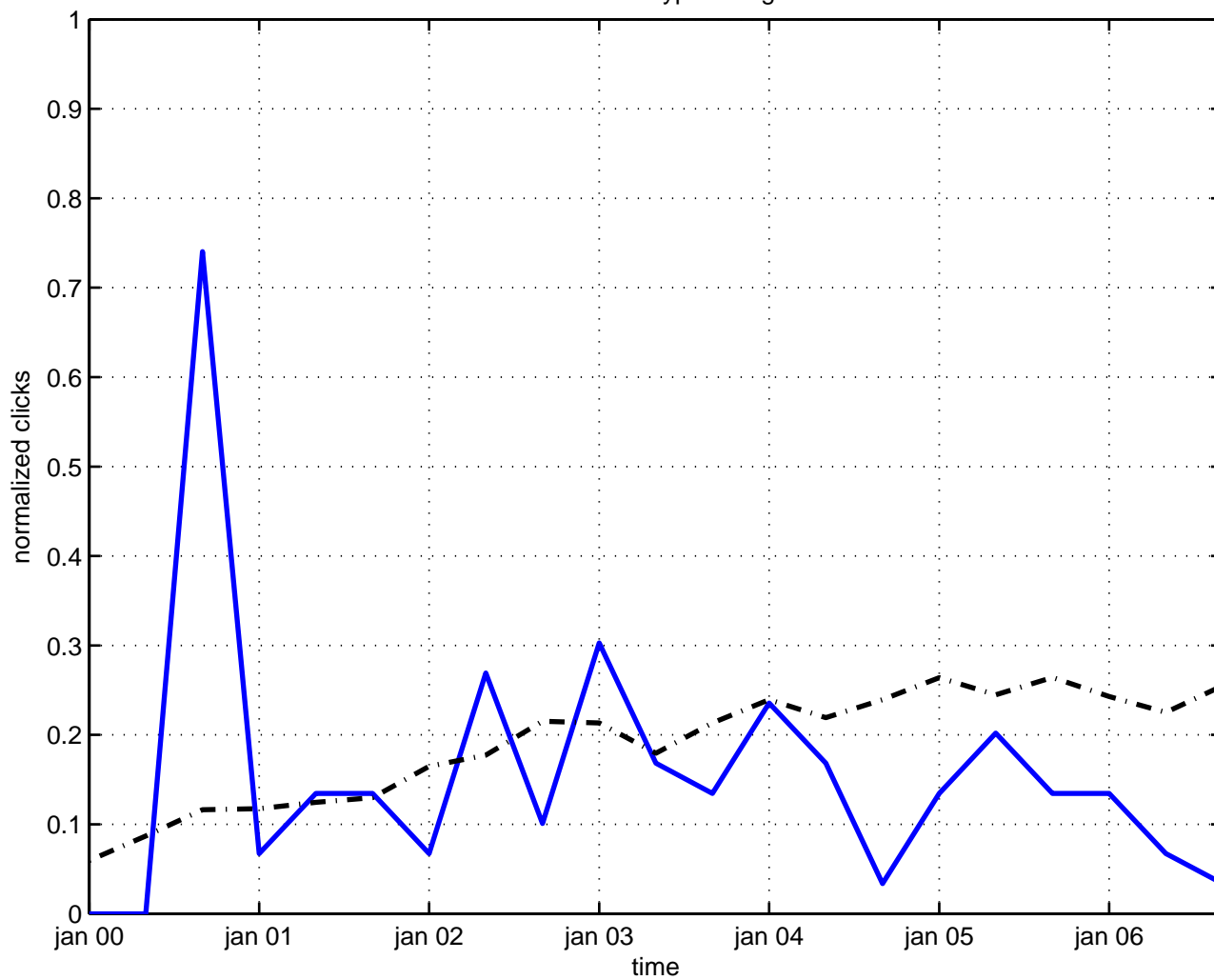
correlation hypercharge
