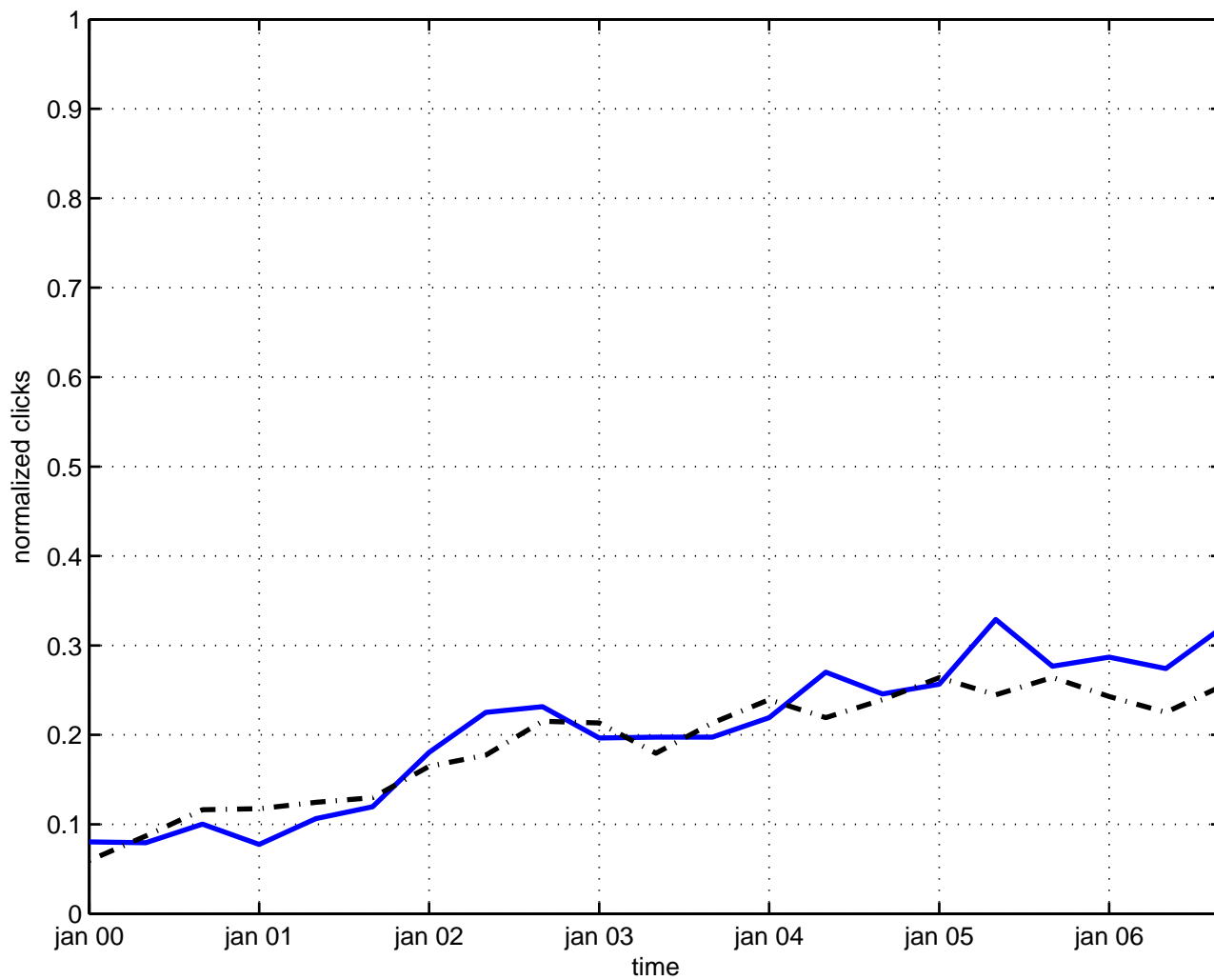
correlation function
