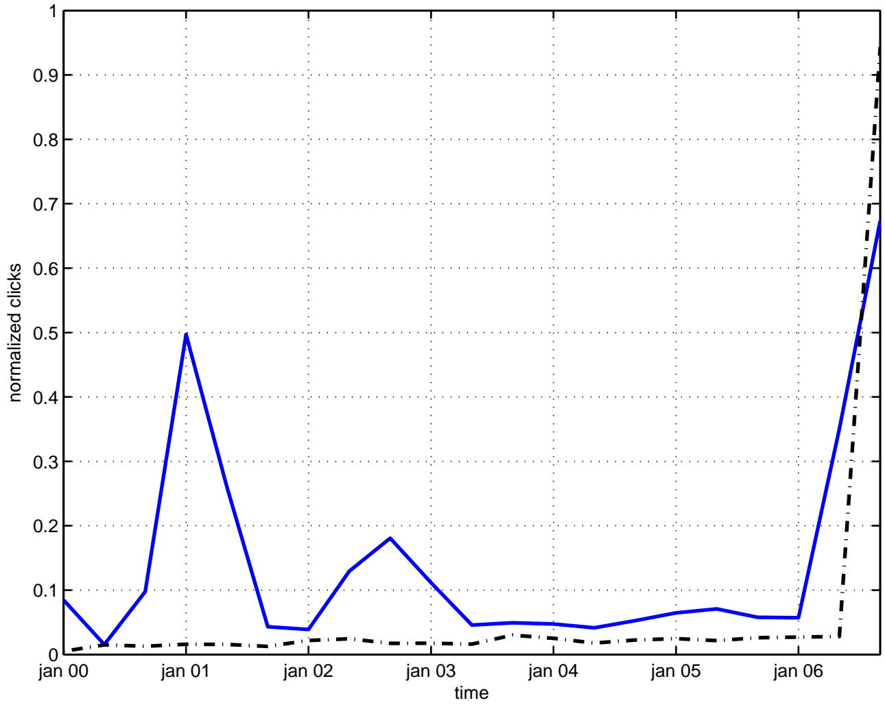
correlation function wilson loop
