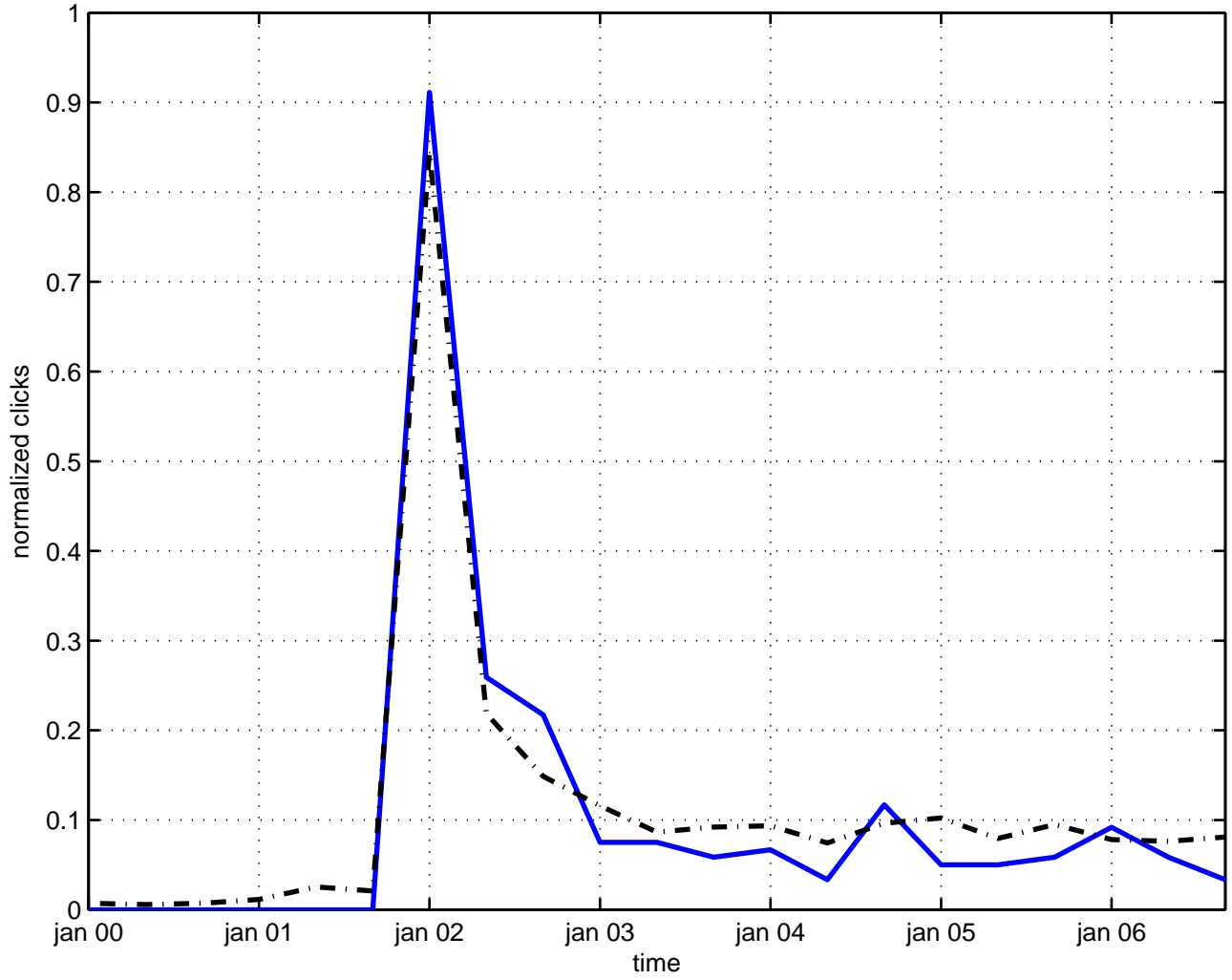
correlation function vortex
