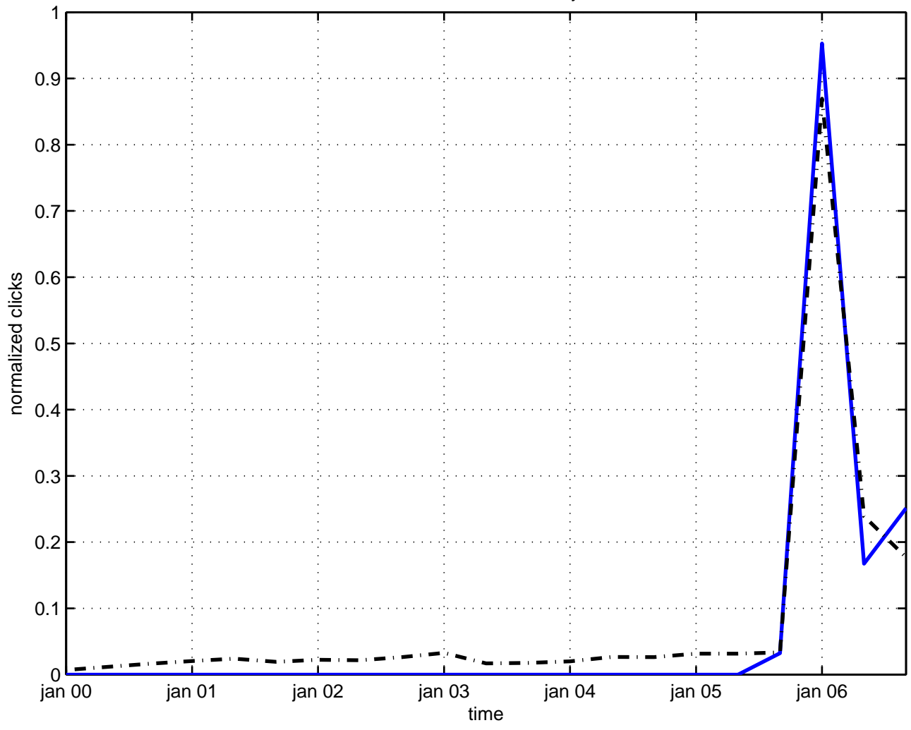
correlation function tachyon
