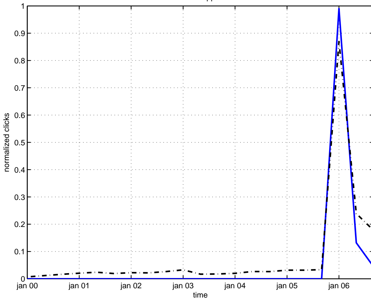
correction wkb approximation
