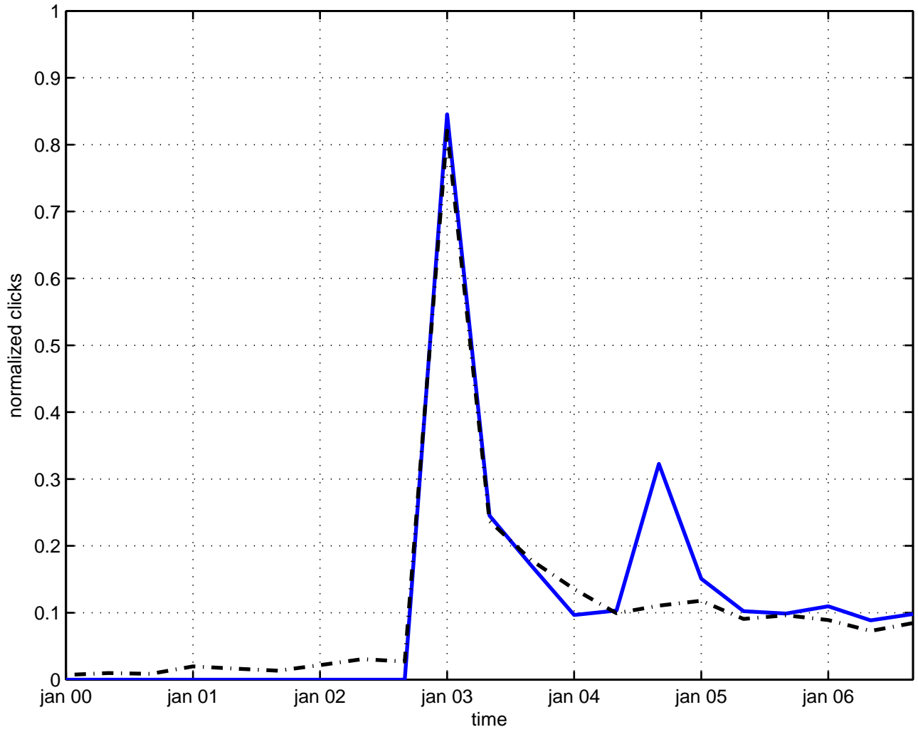
correction sigma model
