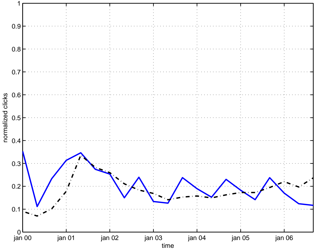
correction quantization
