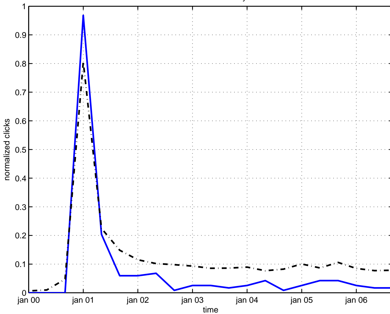
correction m-theory
