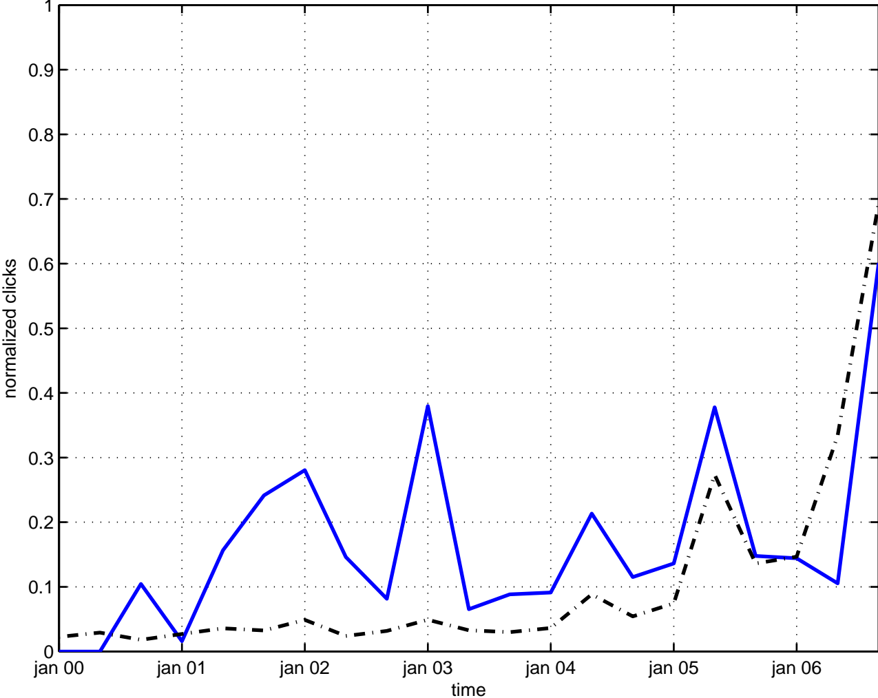
correction instanton
