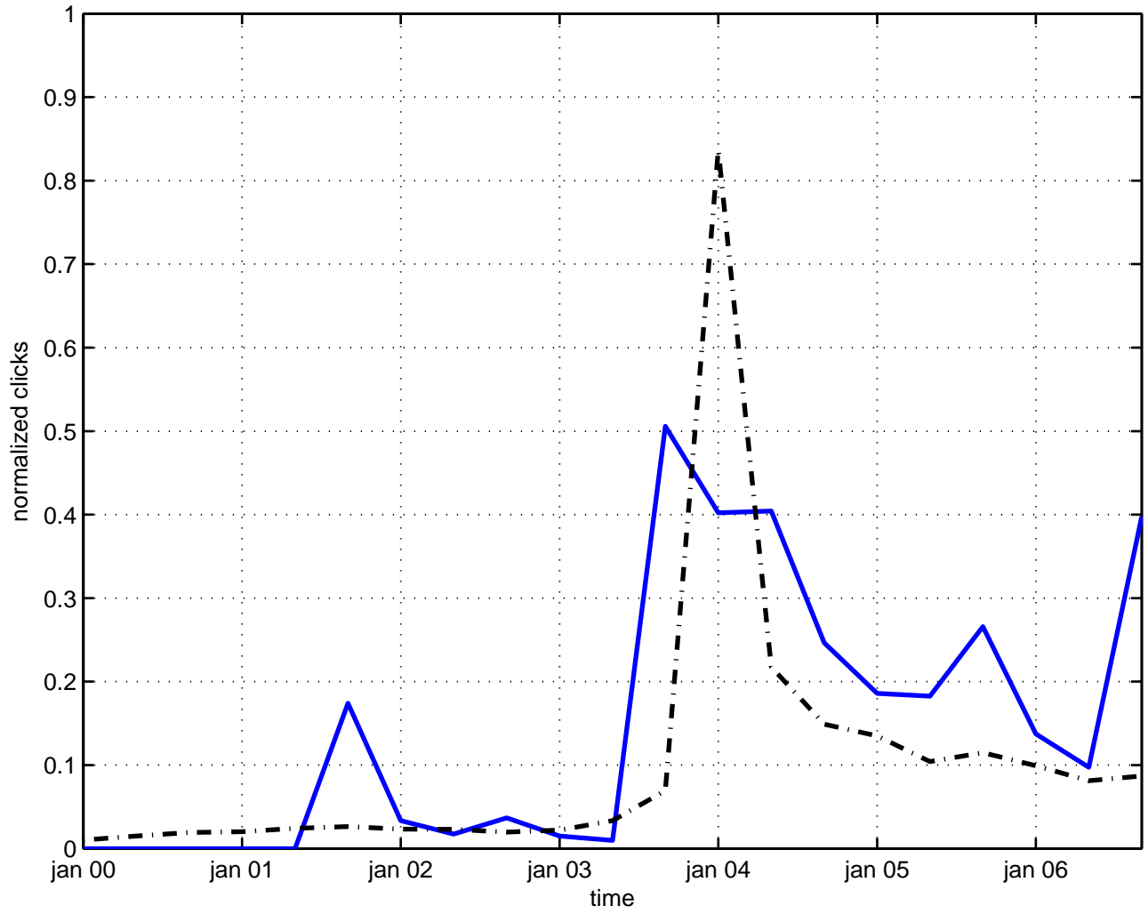
constraint supersymmetry
