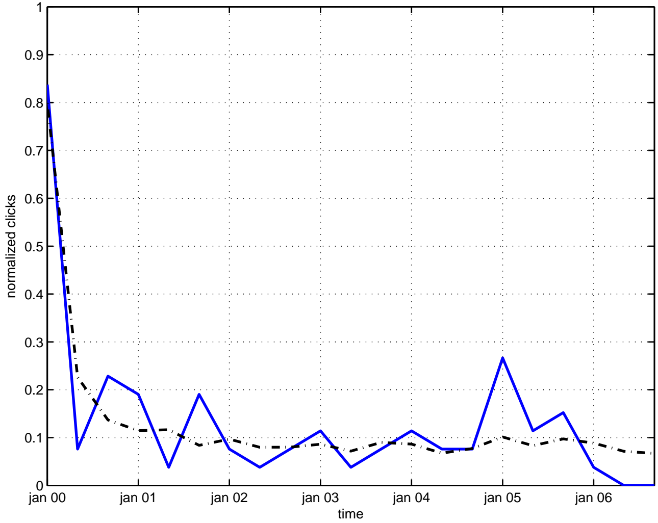
constraint superfield
