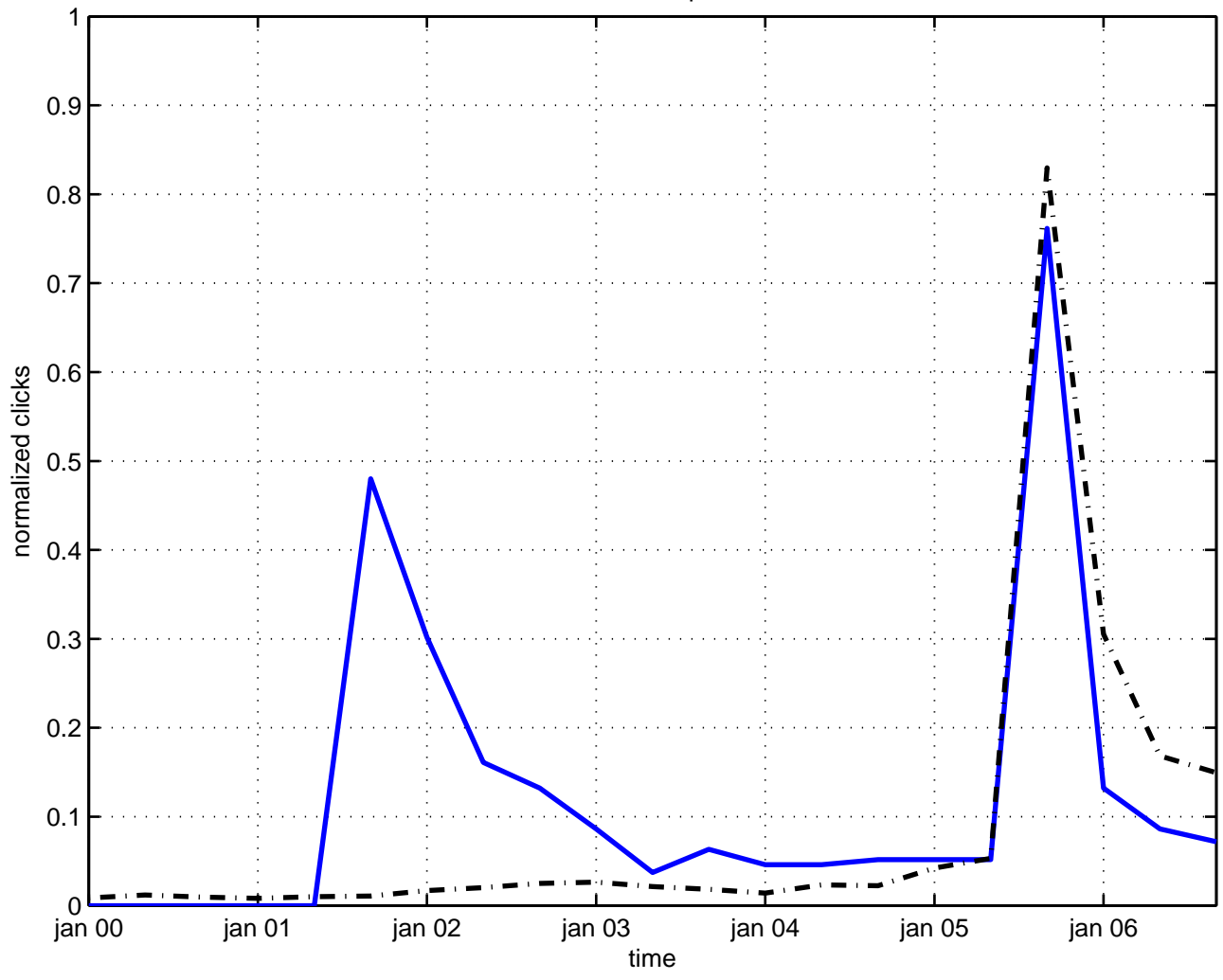
constraint spinor
