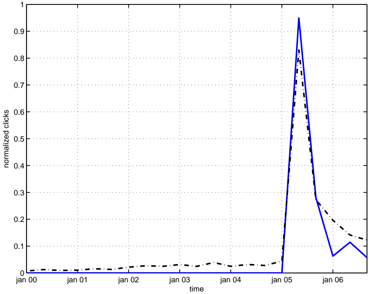
constraint reparametrization
