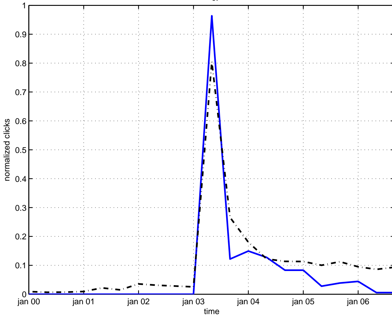
constraint energy-momentum
